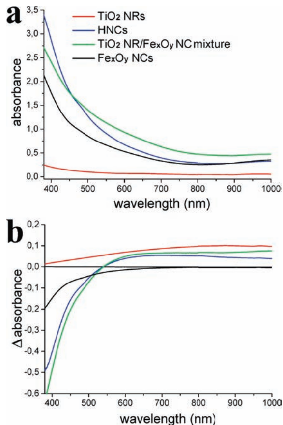
Figure 10. Absorption changes occurring to b -TiO 2 NRs ( \sim 5 nm \times \sim 50 nm), matchstick-like HNCs thereof tipped with \sim 10 nm Fe x O y heads, corresponding NR/Fe x O y NC physical mixtures, and bare \sim 10 nm Fe x O y NCs, upon UV-irradiation in O 2 -free conditions: (a) before and (b) after 60 min irradiation. The spectra in panel b were taken using the unirradiated photocatalyst solution as the reference. Conditions: [TiO 2 ] = 0.72 mM, [Fe 2 O 3 ] = 0.74 mM.
