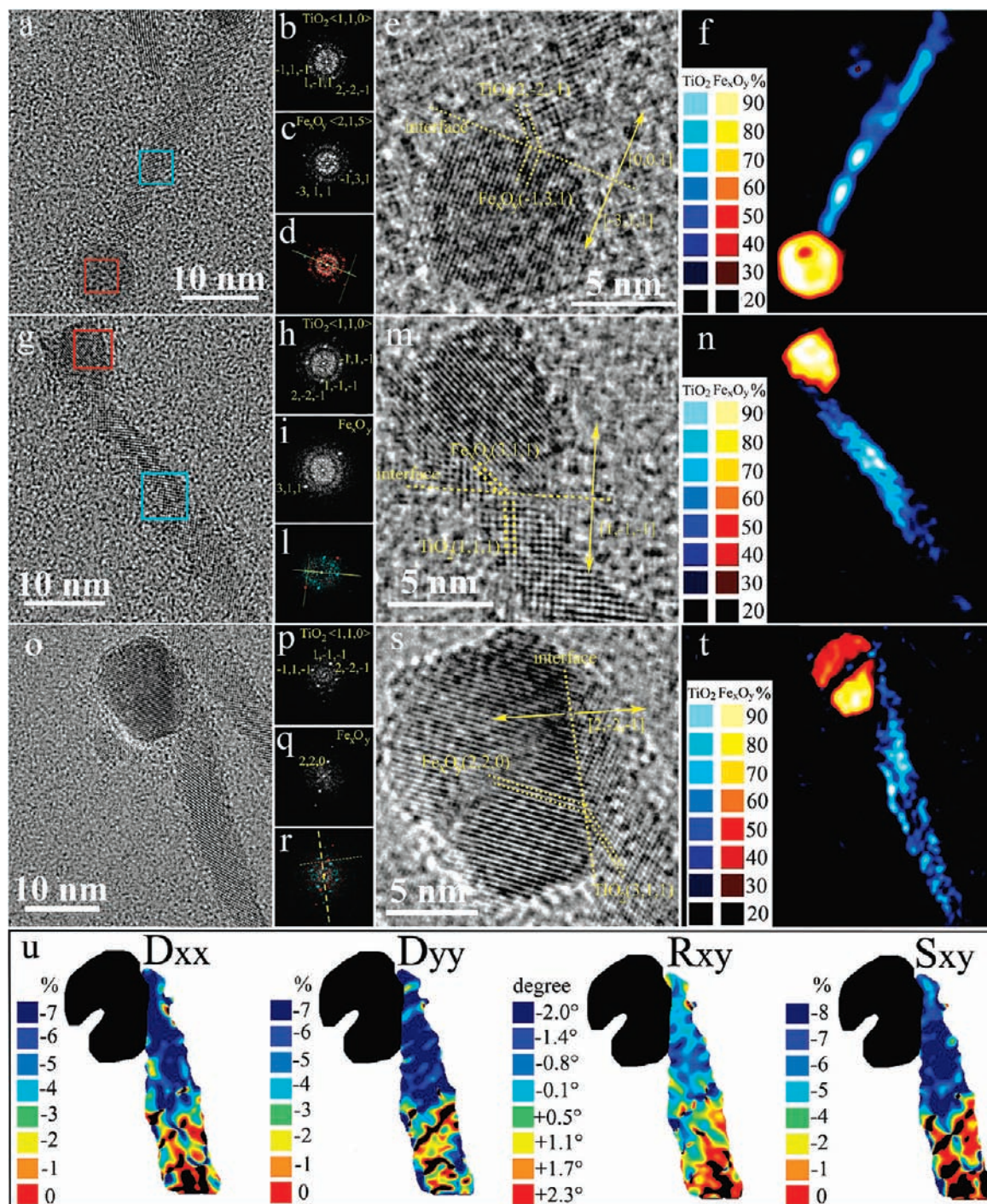
Figure 6. Phase-contrast HRTEM study of HNCs made of asymmetrically \text{Fe}_x\text{O}_y -tipped \text{TiO}_2 nanorods. (a,g,o) HRTEM images of matchstick-like HNCs that incorporate \text{TiO}_2 and \text{Fe}_x\text{O}_y in different relative arrangements. (b,c,h,i,p,q) FFTs calculated from the regions enclosed by the blue and the red boxes in panels a, g, and o, respectively. Brookite \text{TiO}_2 is viewed along the (1,1,0) zone axis in all cases, while a univocal (2,1,5) zone axis can be assigned to inverse spinel cubic \text{Fe}_x\text{O}_y , only for the case in panels a and c. (d,l,r) Joint diffractograms obtained by merging the FFTs in panels b,c, h,i, and p,q, respectively, each traced by a different color. (e,m,s) Magnified views of the matchstick head regions corresponding to the heterostructures in panels a, g, and o, respectively. The relative orientations of the interfacial planes between the two material domains, deduced from the FFT analyses, are marked by dotted yellow lines that correspond to the interface projections in the respective image planes. In panel e, the interface is perpendicular to the [0,0,1]_{\text{TiO}_2} and the [-3,1,1]_{\text{Fe}_x\text{O}_y} directions, while in panels m and s the interface is perpendicular to the [1,-1,-1]_{\text{TiO}_2} and [2,-2,-1]_{\text{Fe}_x\text{O}_y} directions, respectively. The epitaxial relationships between the two lattices are indicated. The interfacial lattice mismatch on the visible one-dimensional projected interfaces can be calculated as:
