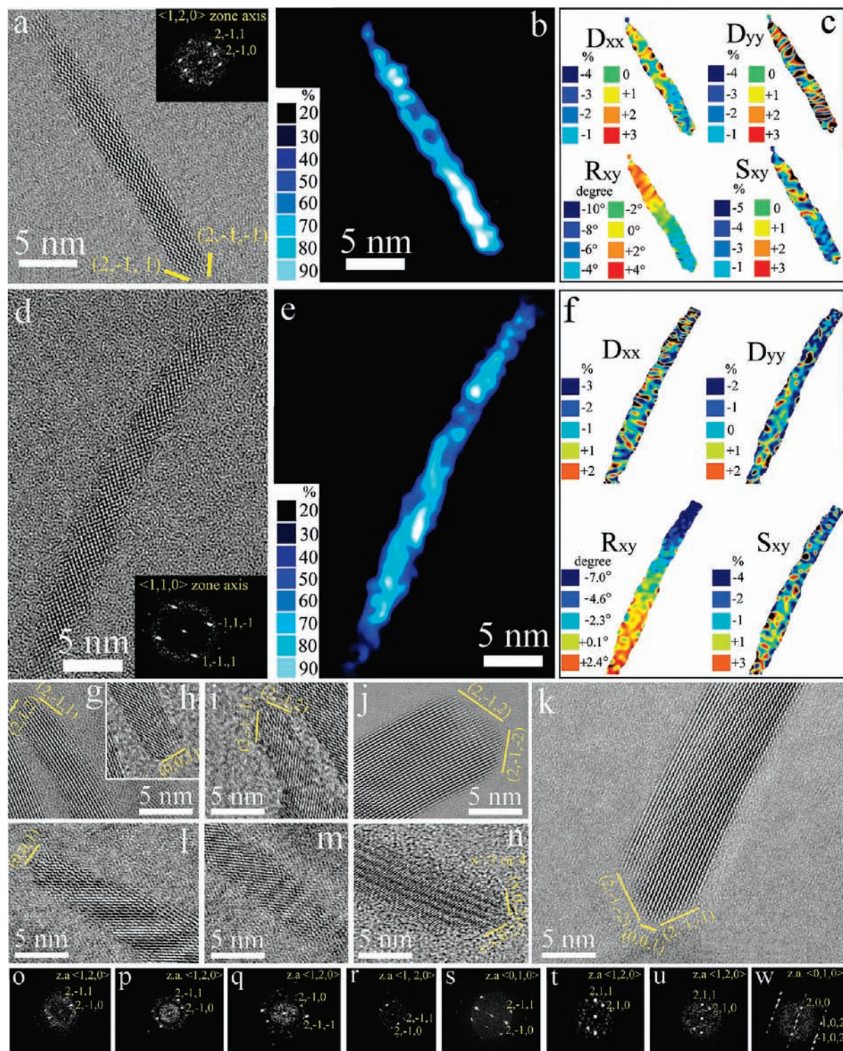
Figure 3. Phase-contrast HRTEM study of b -TiO 2 NR seeds: (a,d) Small-diameter NRs viewed along their \langle 1,2,0 \rangle and \langle 1,1,0 \rangle zone axis, respectively (the insets show the corresponding FFTs). (b,e) False-color crystal-phase amplitude maps obtained by HRTEM contrast analysis of the most intense fringes in the images in panels a and d, respectively. (c,f) False-color strain maps of fringe displacement in the direction perpendicular ( D_{xx} ) and parallel to the long nanorod axis ( D_{yy} ), of fringe rotation ( R_{xy} ), and of shear stress ( S_{xy} ), obtained by GPA analysis of the most prominent fringes in the HRTEM images in panels a and d, respectively. (g–n) Magnified HRTEM views of the apices of differently sized NRs. (o–w) FFTs relative to the nanostructure sections shown in panels g–n, respectively.
