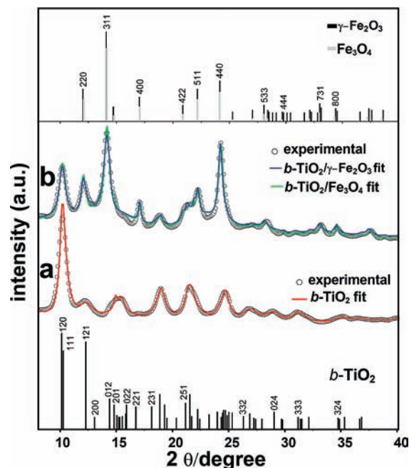
Figure 2. Representative SR-XRD patterns of \sim 5 \pm 0.8 nm \times \sim 60 \pm 4 nm b -TiO 2 NR seeds (curve a); b -TiO 2 /Fe 3 O 4 HNCs, grown from such NR seeds, which are functionalized with Fe 3 O 4 domains of \sim 10 nm (curve b), along with the reference pattern for bulk TiO 2 brookite ( b -TiO 2 ), magnetite (Fe 3 O 4 ), and maghemite ( \gamma -Fe 2 O 3 ). The experimental curves (black) are compared to Rietveld-based fits accomplished assuming the existence of b -TiO 2 (curve a) or mixtures of b -TiO 2 / \gamma -Fe 2 O 3 or b -TiO 2 /Fe 3 O 4 (curve b). The refined cell parameters calculated were as follows: a = 9.168964 Å, b = 5.454103 Å, c = 5.139221 Å for b -TiO 2 in the HNCs and a = 9.246865 Å, b = 5.417928 Å, c = 5.182731 Å for b -TiO 2 in the starting NRs, respectively. The GOF indicators were < 2-3 in all cases. Any possible anatase contamination was verified to be of the order of 2–3%, which is within the accuracy of the fitting procedure and, therefore, considered to be negligible.
