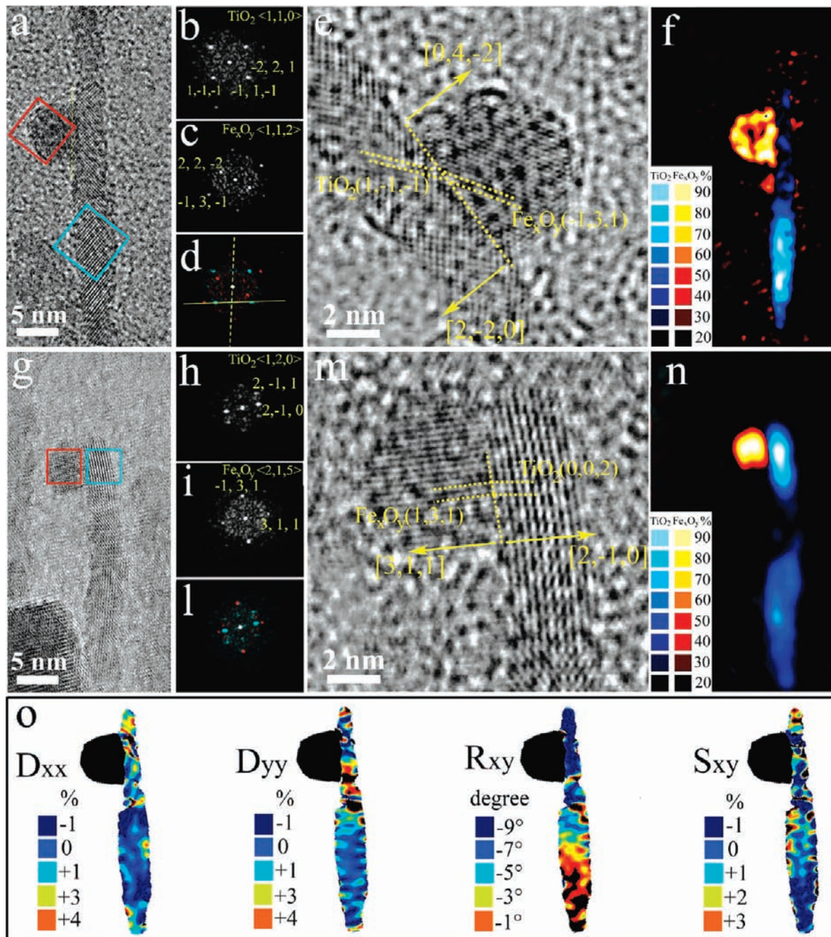
Figure 7. Phase-contrast HRTEM study of HNCs made of TiO 2 nanorods decorated with Fe x O y domains on their longitudinal sidewalls: (a,g) HRTEM images of heterostructures in different relative configurations. (b,c,h,i) Corresponding fast Fourier transform (FFT) analyses of the regions enclosed by the blue and the red boxes in panel a, which correspond to brookite TiO 2 viewed along the \langle 1,1,0 \rangle and \langle 1,2,0 \rangle zone axis, and inverse spinel cubic Fe x O y down the \langle 1,1,2 \rangle and \langle 2,1,5 \rangle zone axis, respectively. (d,l) Joint diffractograms obtained by merging the FFTs in panels b,c and h,i, respectively, each traced by a different color. (e,m) Magnified HRTEM view of the matchstick head in panels a,g. The relative orientations of the interfacial planes between the two material domains are marked by dotted yellow lines. In panel e, the interface is perpendicular to the [2, -2, 0]_{\text{TiO}_2} and [0, 4, -2]_{\text{Fe}_x\text{O}_y} directions, while in panel m the interface is approximately perpendicular to the [2, -1, 0]_{\text{TiO}_2} and [3, 1, 1]_{\text{Fe}_x\text{O}_y} directions, respectively. The lattice mismatch can be calculated as:
