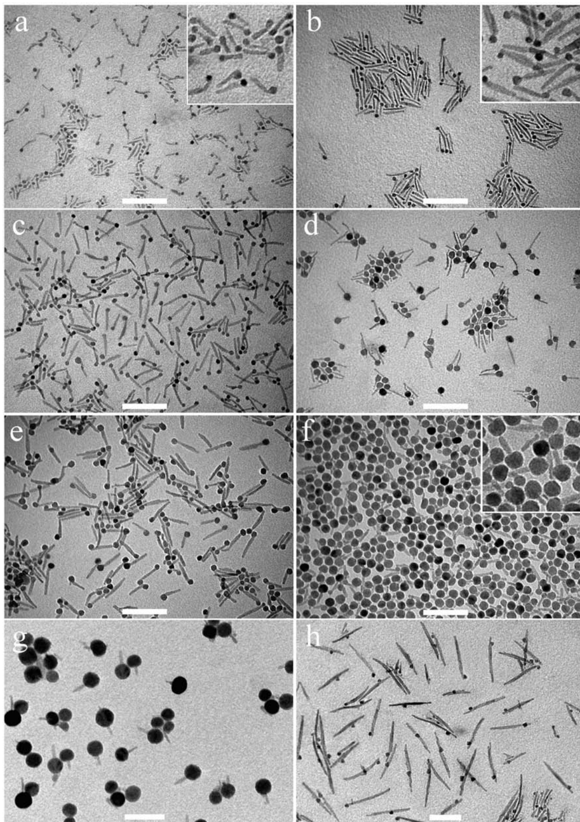
Figure 4. Representative low-magnification TEM overviews of (a–g) matchstick-shaped and (h) longitudinally decorated HNCs synthesized by reacting tapered b -TiO 2 NR seeds with different sizes and aspect ratios with varying amounts of Fe(CO) 5 in OLAC:OLAM:DDIOL:ODE mixtures (white scale bar = 100 nm). The relevant reaction parameters are summarized in Table 1.
