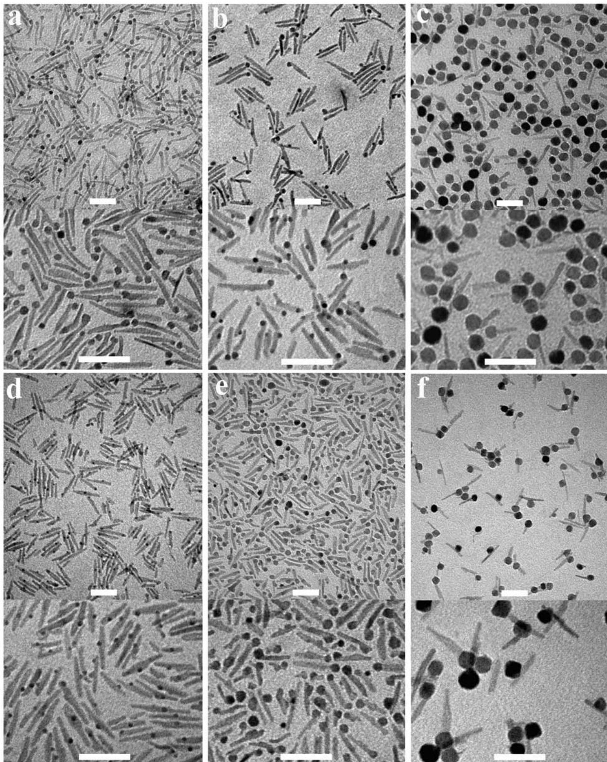
Figure 5. Representative low-magnification TEM images of HNCs achieved in precursor-injection-modulated experiments: (a,b,d) HNCs obtained from the same NR seeds upon adding progressively lower \text{Fe}(\text{CO})_5 amounts in the fast-injection step; (c,e,f) HNCs deriving from the heterostructures shown in panels b and d, respectively, after slow supply of extra precursor feedstock solution (the white scale bar = 50 nm). The relevant reaction conditions are summarized in Table 2.
