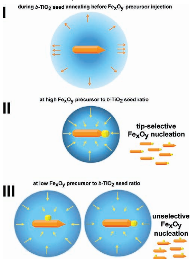
Scheme 2. Sketch of the Proposed Diffusion-Controlled Mechanism of HNC Topology Selection as a Function of the b -TiO 2 NR Seed to Fe x O y Precursor Ratio a
