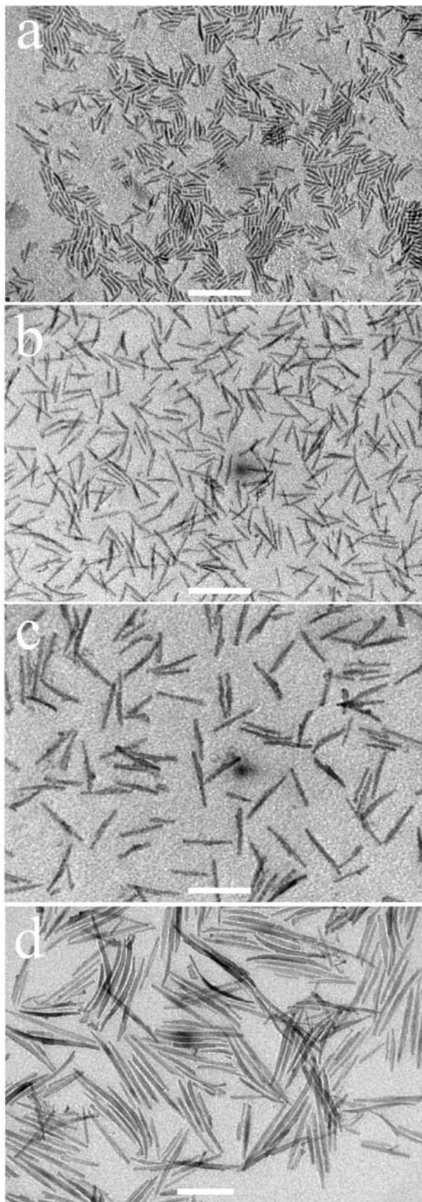
Figure 1. Low-magnification TEM overview of tapered b -TiO 2 NRs (seeds) with different geometric parameters synthesized by reacting a total amount of 1 mmol (a), 8 mmol (b), 14 mmol (c), and 18 mmol (d) of TiCl 4 , respectively, in OLAM:OLAC:ODE mixtures (white scale bar = 100 nm).
