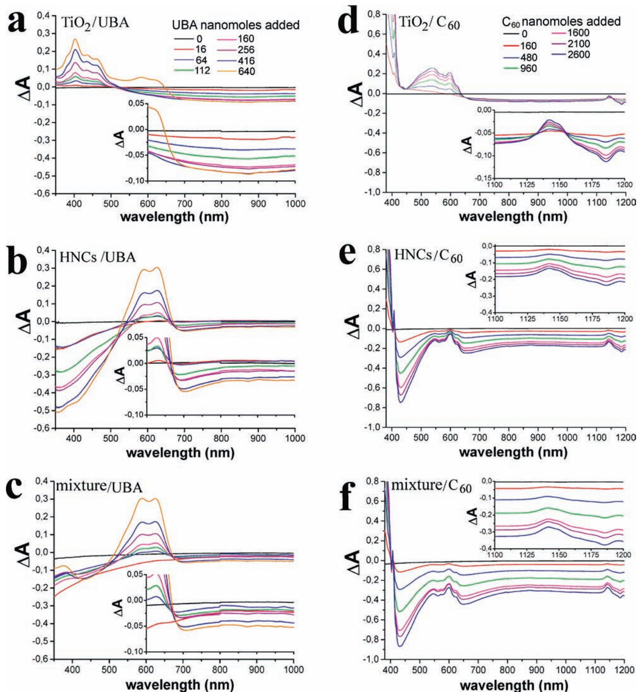
Figure 11. Electron titration experiments: absorption changes occurring to (a,d) preirradiated b -TiO 2 NRs ( \sim 5 \text{ nm} \times \sim 50 \text{ nm} ), (b,e) matchstick-like HNCs thereof, tipped with \sim 10 \text{ nm} Fe x O y heads, and (c,f) corresponding NR/Fe x O y NC physical mixtures upon successive additions of UBA (a–c) or of C 60 (d–f) in O 2 -free conditions. The spectra were taken using the irradiated photocatalyst solution as the reference (cf., Figure 10b) and were corrected by the relevant dilution factor. Conditions: [TiO 2 ] = 0.72 mM, [Fe 2 O 3 ] = 0.74 mM; preirradiation time = 60 min (note that the small kinks detectable at 800 nm in some cases are artifacts due to light source switching in the spectrophotometer).
