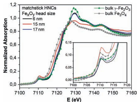
Figure 8. Normalized XANES spectra of matchstick-like HNCs made of \sim 5 \times 50 nm b - \text{TiO}_2 sections tipped with \text{Fe}_x\text{O}_y heads of \sim 6 , \sim 15 , and \sim 17 nm, respectively, along with the spectra of bulk \gamma - \text{Fe}_2\text{O}_3 and \text{Fe}_3\text{O}_4 references. The inset shows a magnified view of the pre-edge peak region.
